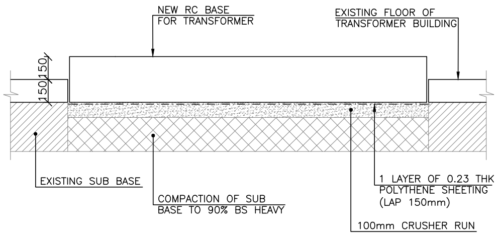
TYPICAL DETAIL FOR TRANSFORMER BASE (SCALE 1:25)
